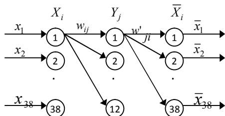
Fig. 2 – NPCA neural network.
